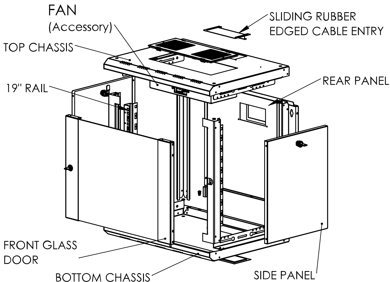
Exploded view
