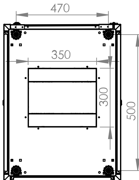
Bottom view
