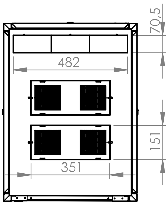
Top view
