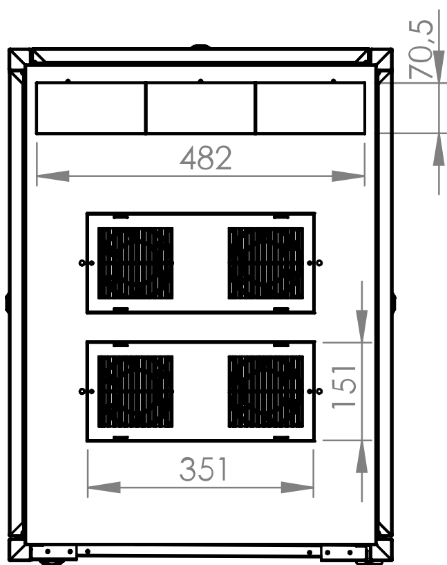
Top view
