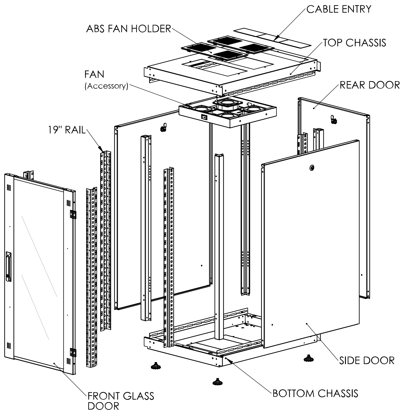
Exploded view
