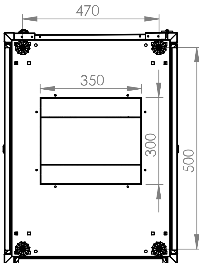
Bottom view
